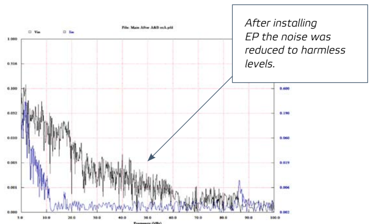
Figure 2: Current & Voltage Noise After EP
